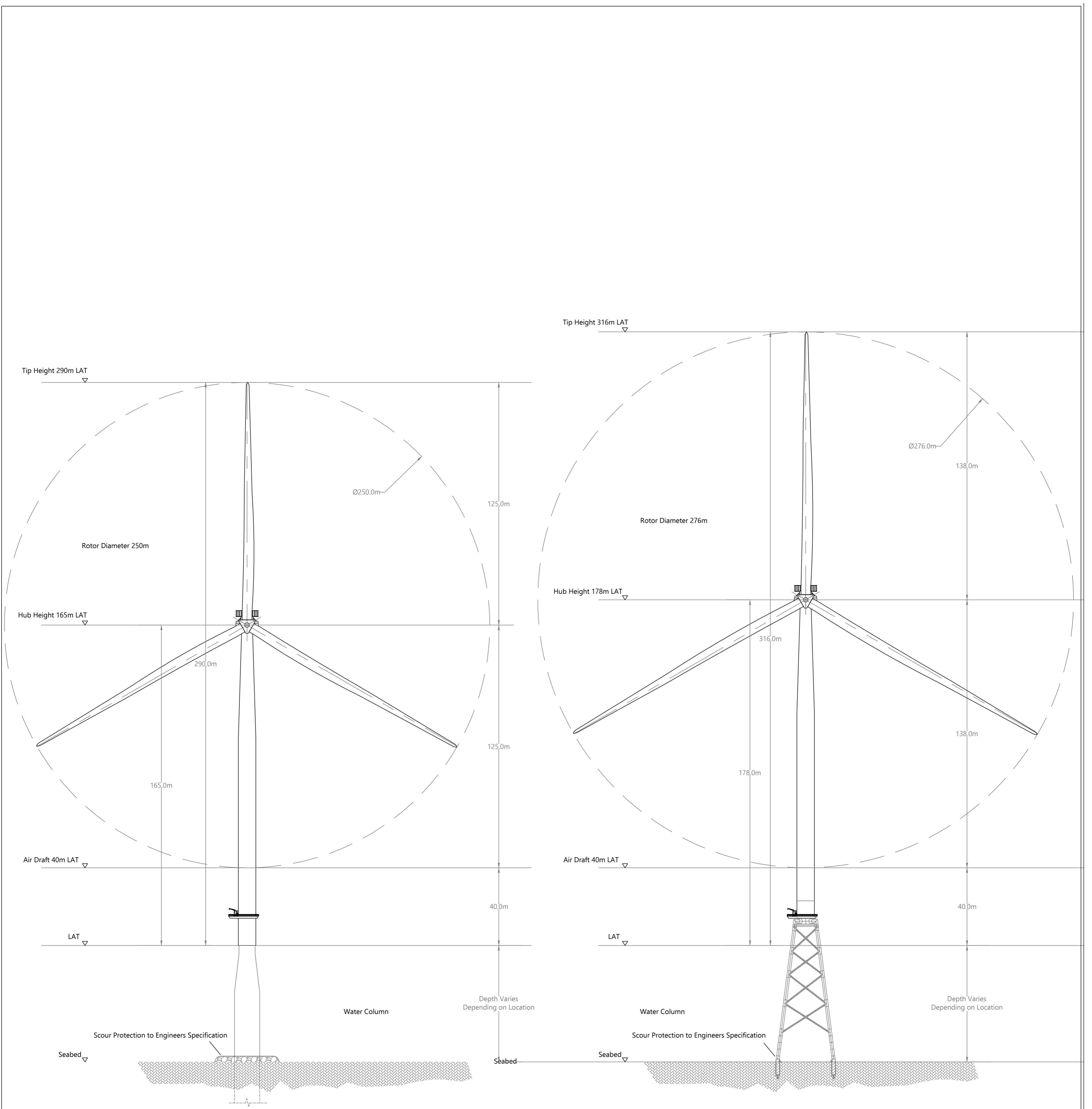
Proposed Monopile Type Foundation Option 1
