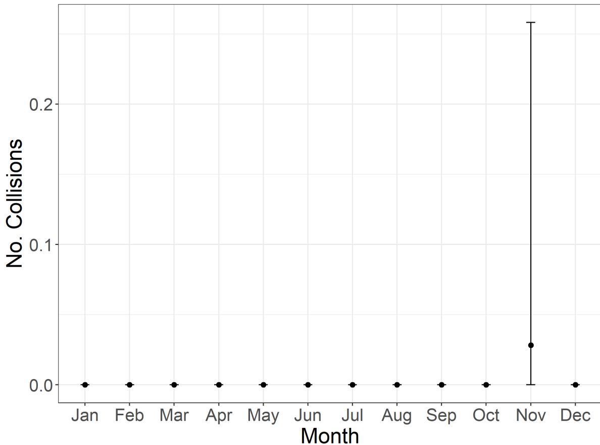
Figure A3.2 Mean monthly collisions predicted for black-headed gull for Project Option 1 Band Option 2. Error bars display the upper and lower confidence intervals of monthly collision (replaces Figure 3.2 of Appendix 15.3 of the 2024 EIAR).
