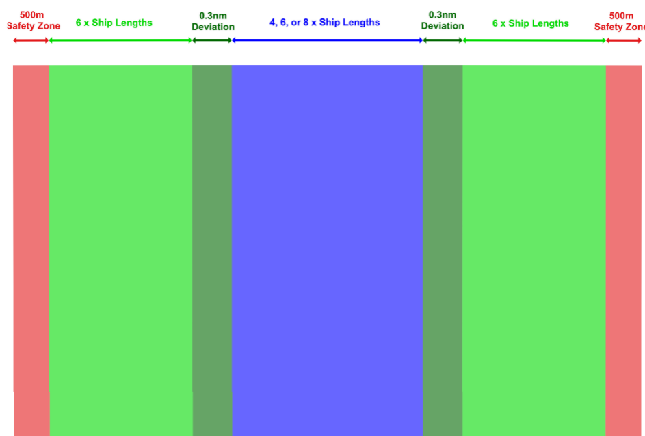
Figure E.13 Gap Methodology Applied Based on PIANC and MARIN
