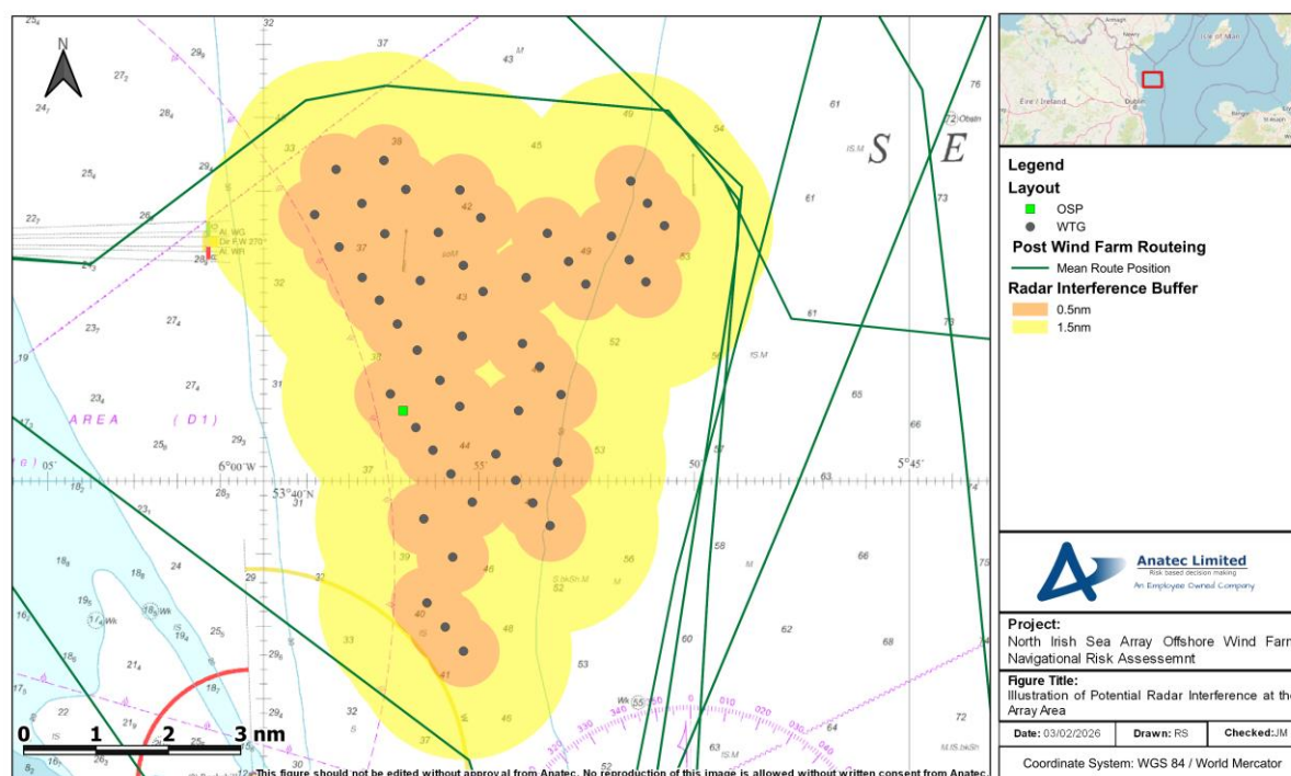
Figure A14.4 Illustration of Potential Radar Interference at the Array Area
