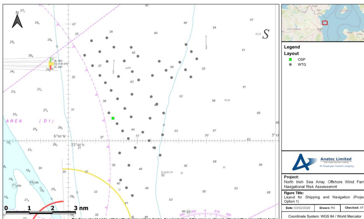
Figure A6.4 Layout for Shipping and Navigation (Project Option 1)
