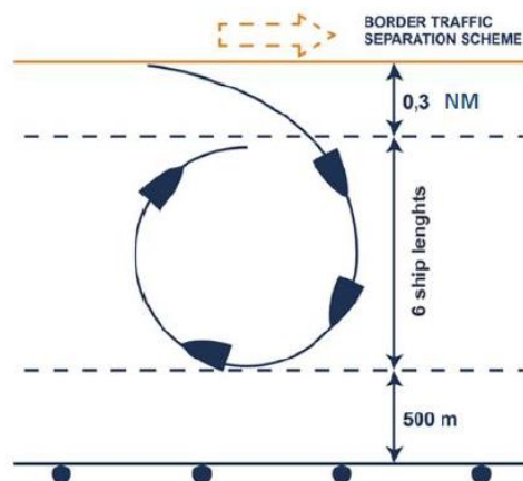
Figure E.12 Sea Space Required for Full Round Turn (PIANC, 2018)
