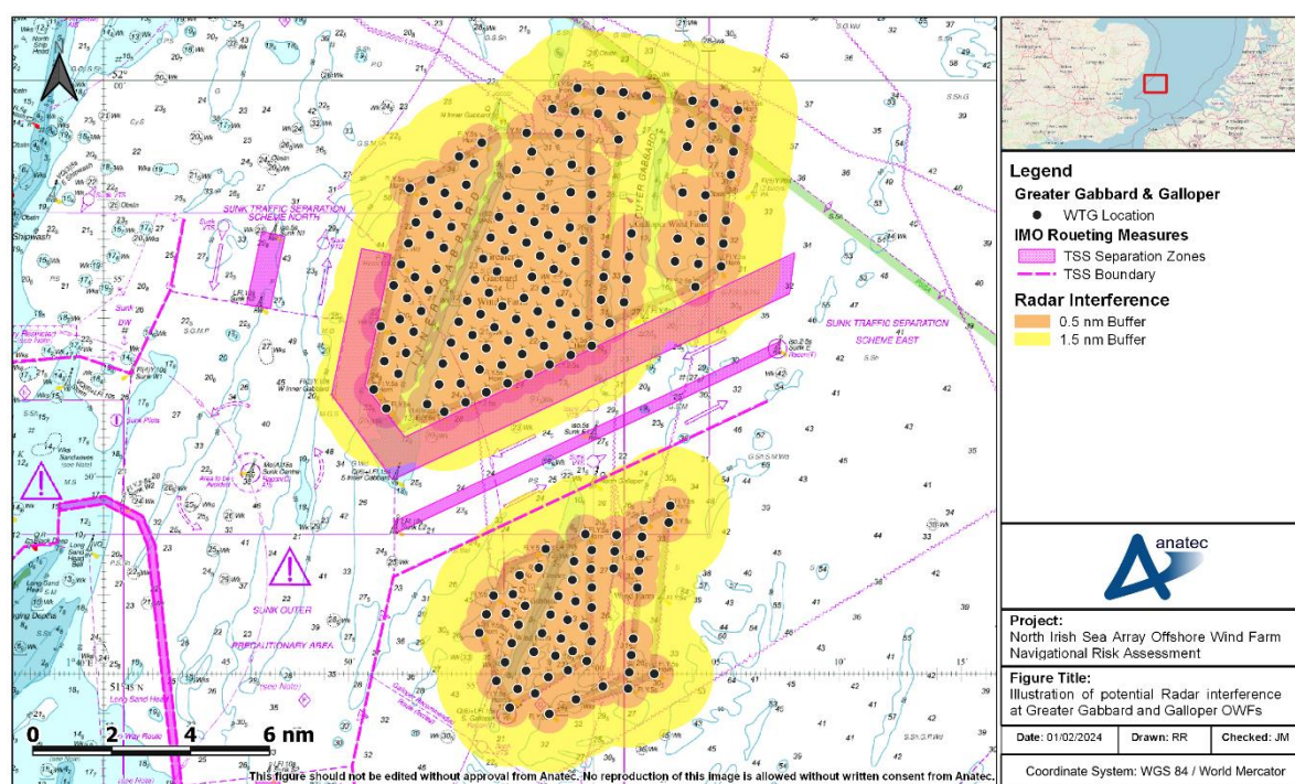
Figure A14.3 Illustration of potential Radar interference at Greater Gabbard and Galloper Offshore Wind Farms
