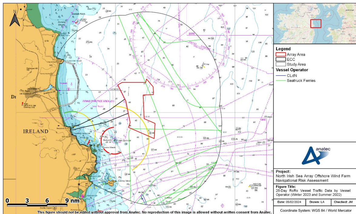
Figure A10.10 28-Day RoRo Vessel Traffic Data by Vessel Operator (Summer 2022 and Winter 2023)
