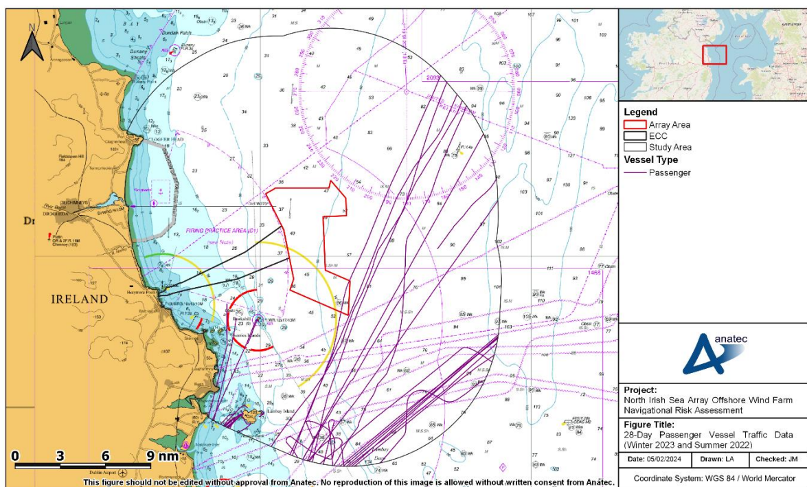
Figure A10.13 28-Day Passenger Vessel Traffic Data (Summer 2022 and Winter 2023)
