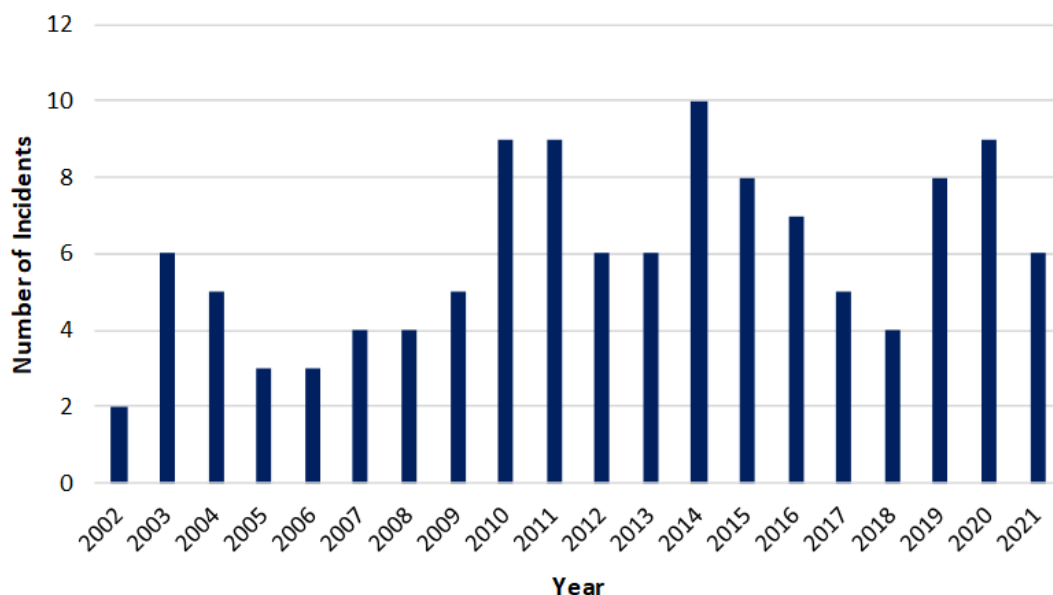
Figure B.12 MAIB Contact Incidents per Year within UK Waters (2002 to 2021)
