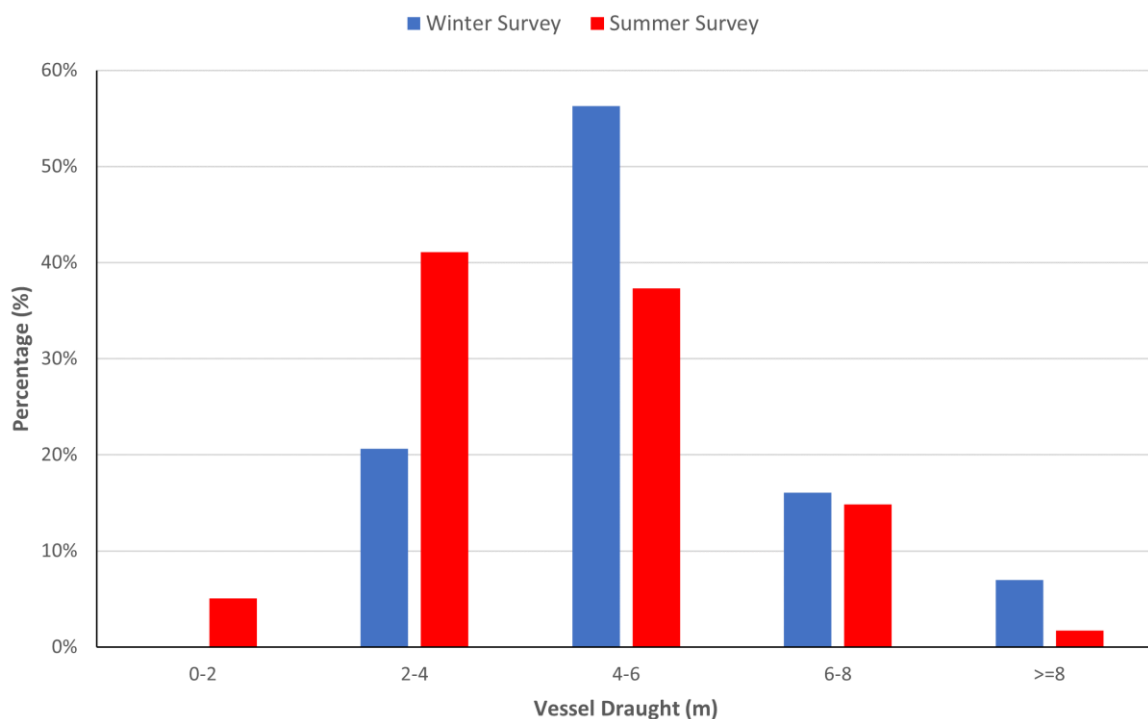
Figure A10.19 28-Day Vessel Draught Distribution by Survey Period (Summer 2022 and Winter 2023)
