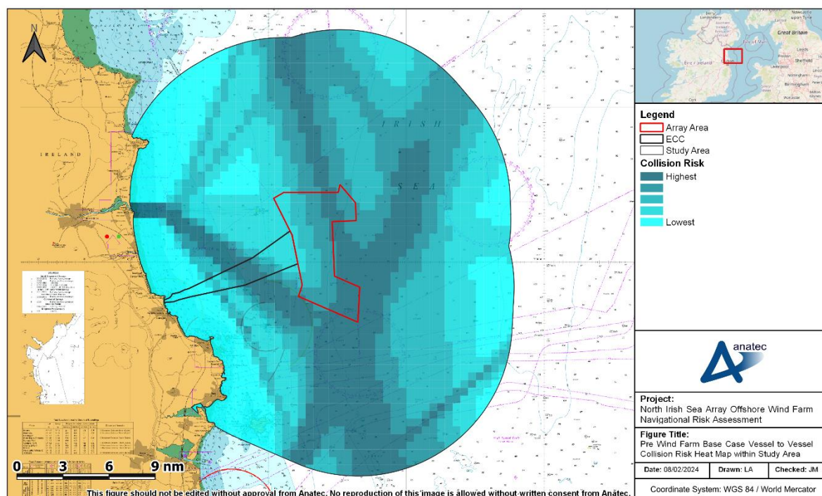
Figure A17.2 Pre Wind Farm Base Case Vessel to Vessel Collision Risk Heat Map within Study Area
