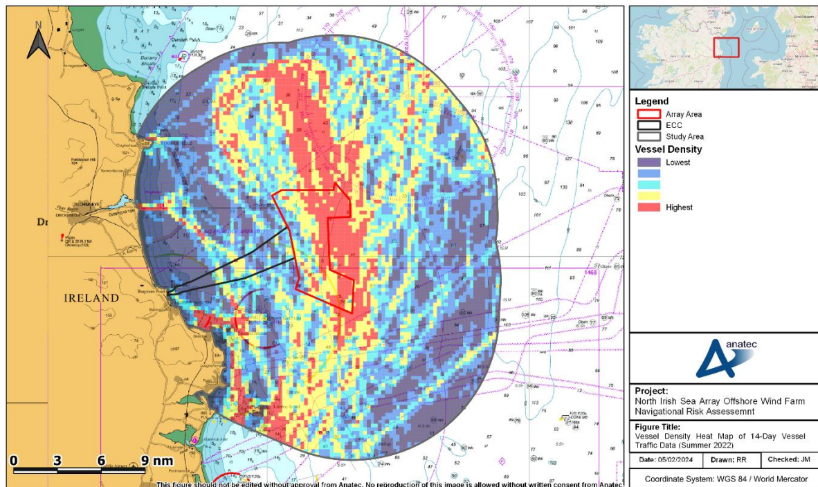
Figure A10.2 Vessel Density Heat Map of 14-Day Vessel Traffic (Summer 2022)
