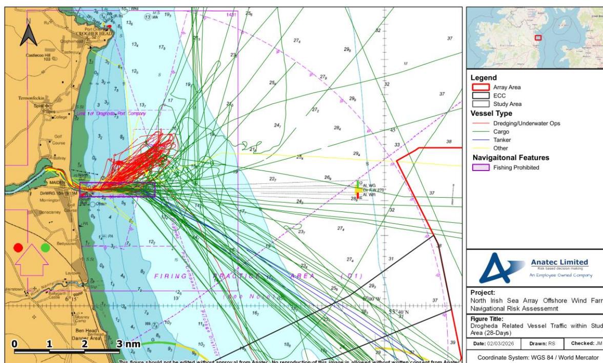
Figure A11.3 Drogheda Related Vessel Traffic within Study Area (28-Days)
