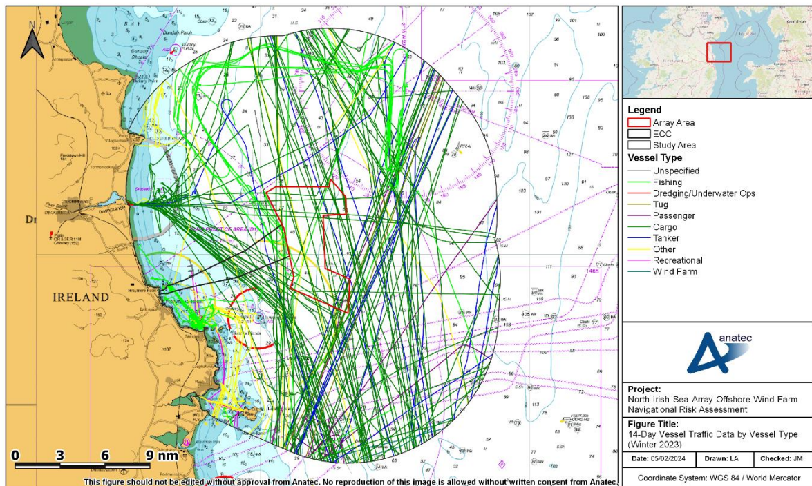
Figure A10.3 14-Day Vessel Traffic Data by Vessel Type (Winter 2023)
