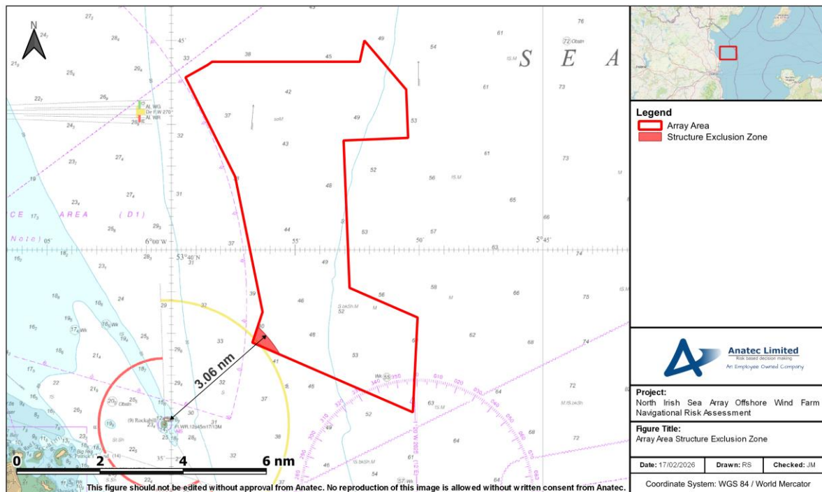
Figure A6.2 Array Area Structure Exclusion Zone
