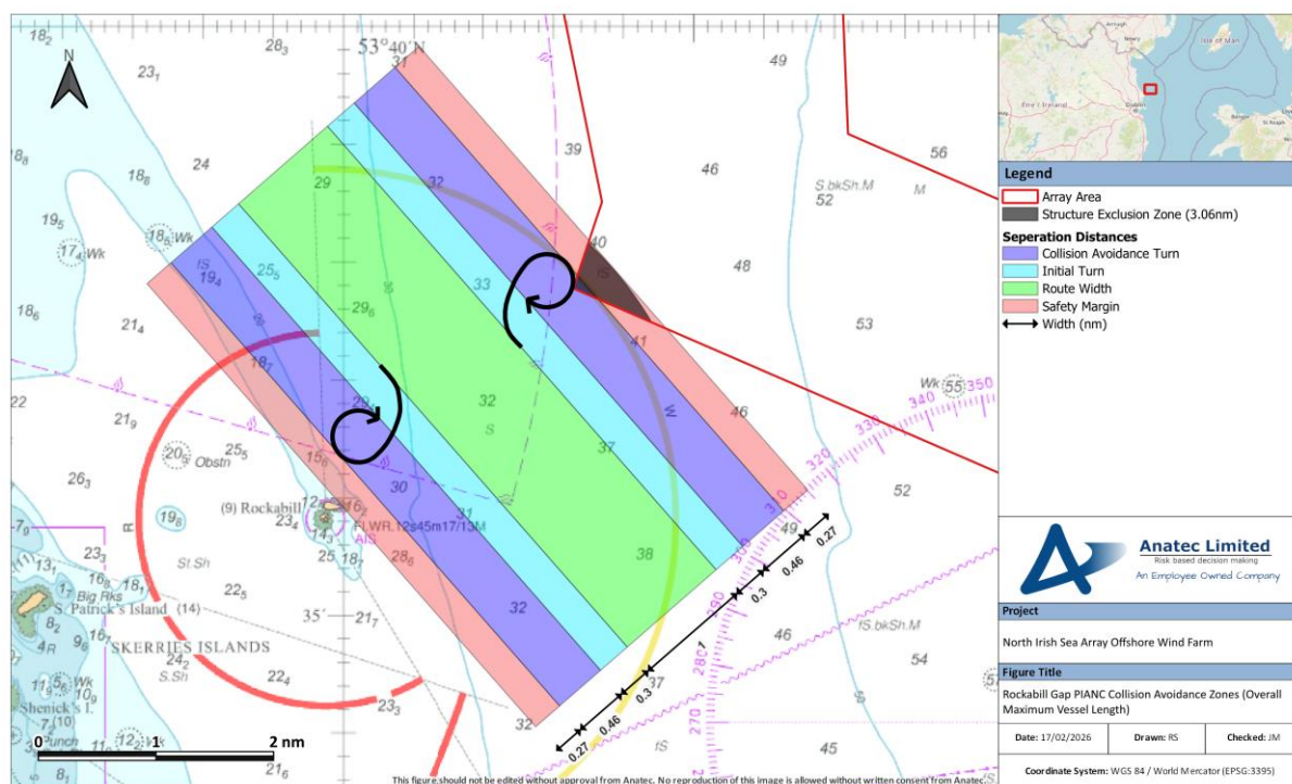
Figure E.14 Rockabill Gap PIANC Collision Avoidance Zones (Maximum Vessel Length)
