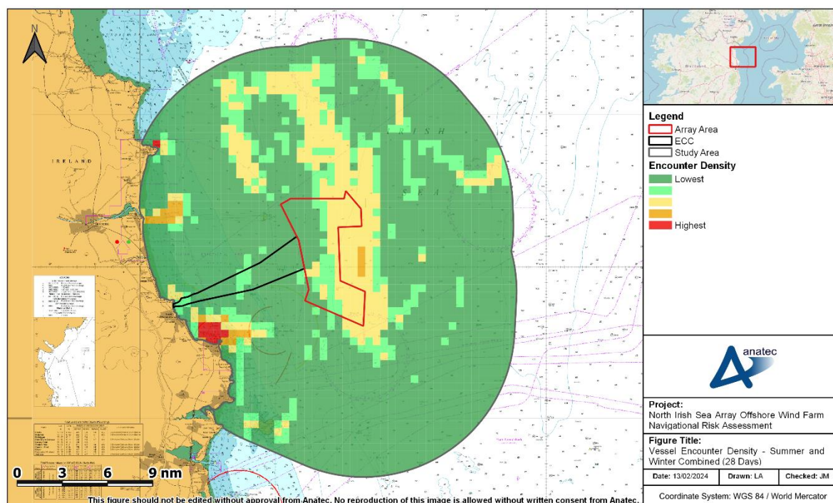
Figure A17.1 Vessel Encounter Density – Summer and Winter Combined (28–Days)
