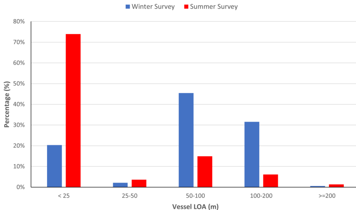
Figure A10.17 28-Day Vessel Length Distribution by Survey Period (Summer 2022 and Winter 2023)
