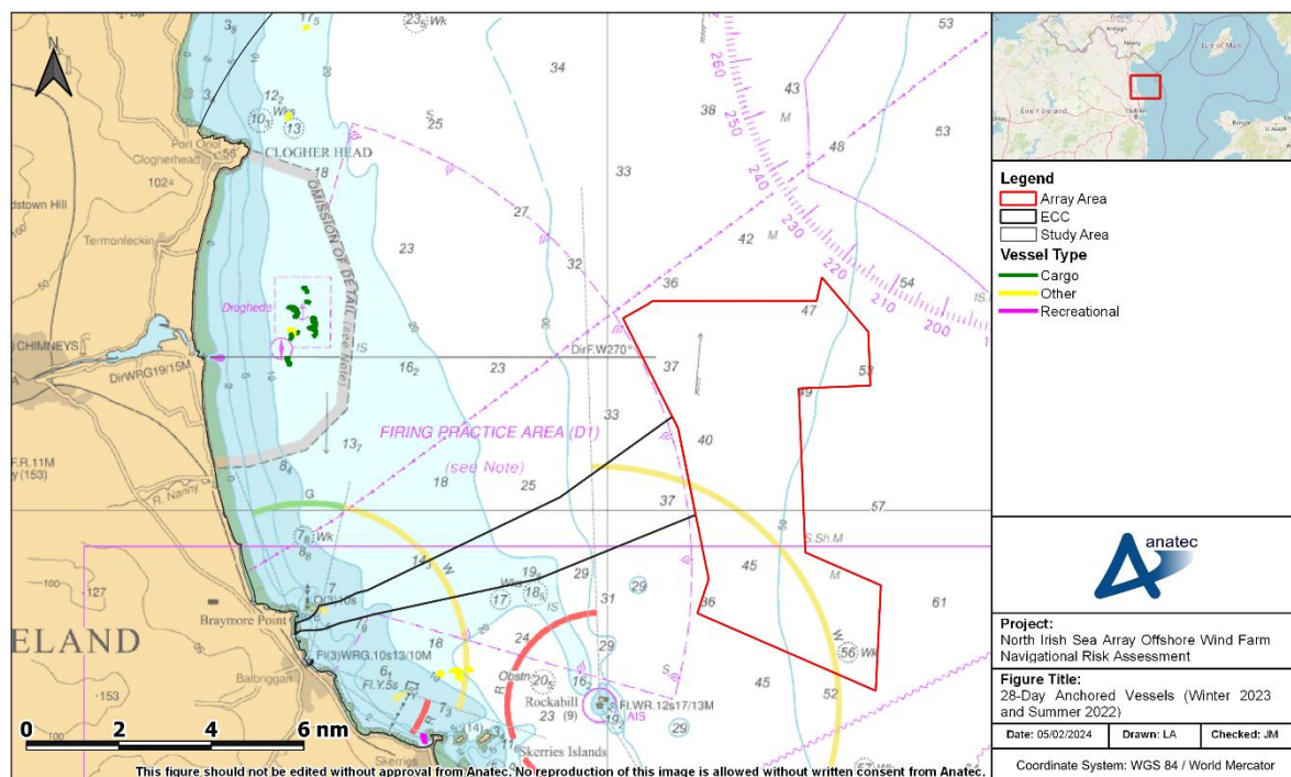
Figure A10.15 28-Day Anchored Vessels (Summer 2022 and Winter 2023)
