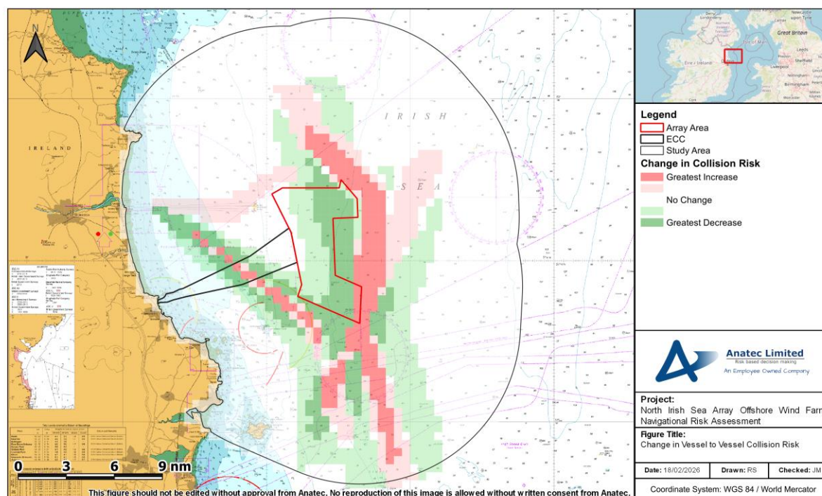
Figure A17.5 Change in Vessel to Vessel Collision Risk
