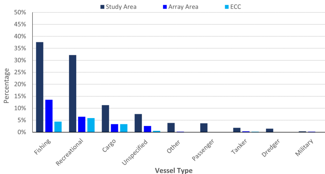
Figure A10.7 Main Vessel Type Distributions (Summer 2022)
